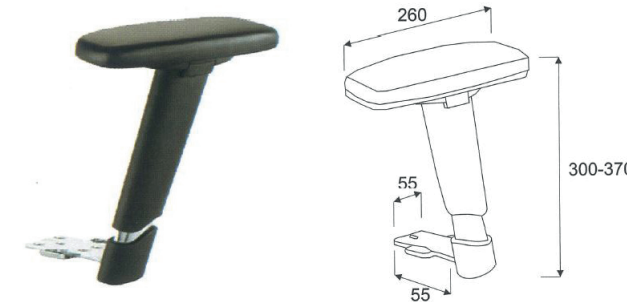
Adjustable Chrome 3D Armrests YA 3683 0010
