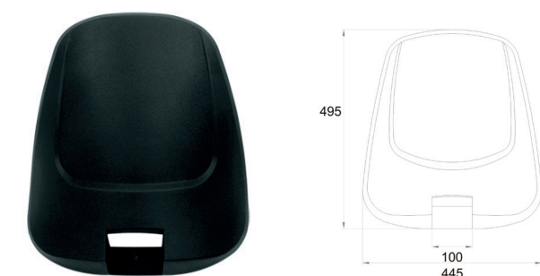
Rose High Plastic Back
