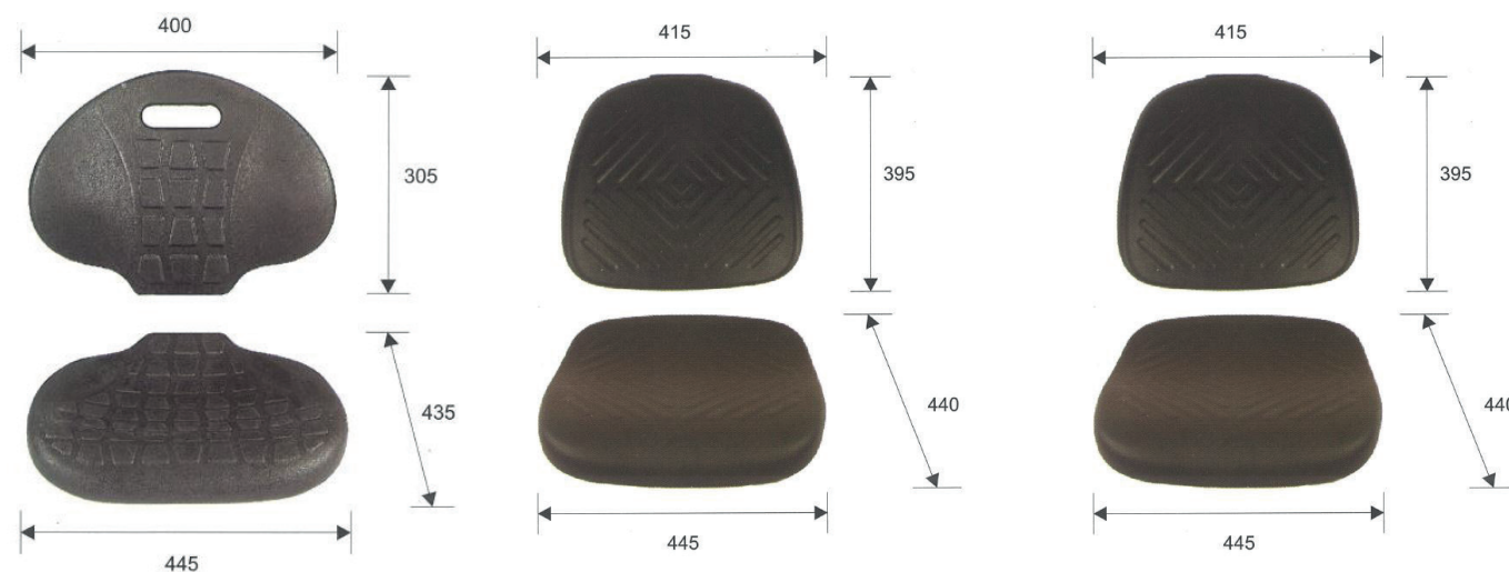
Standard YS 9004 1006 (Back) YS 9504 1006 (Seat)
