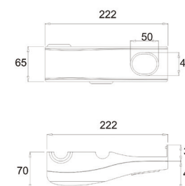
Mechanism Cover YS 1020 1001
