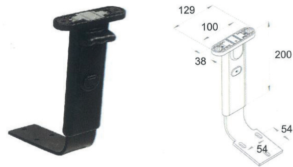
Adjustable Armrests YA 3173 1001
