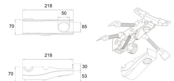
Mechanism Cover YS 1021 1001
