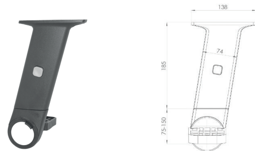
Folding Adjustable Armrests YA 3203 1001
