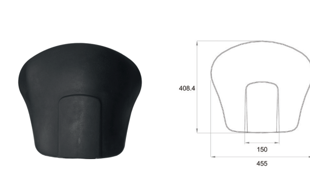
Mayflower Medium Plastic Back
