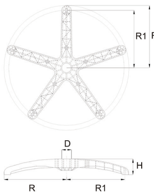
Spider Nylon Base YB 1130 1001 (23") YB 1132 1001 (25") YB 1135 1001 (27")
