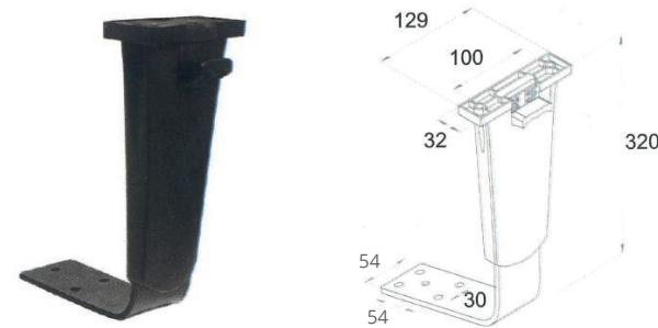
Adjustable Armrests YA 3193 1001
