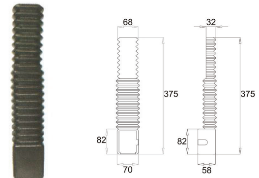
Plastic Gaiter YE 5044 1004
